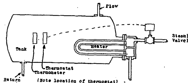
FIG. 65. STEAM HEATED SERVICE WATER HEATER
