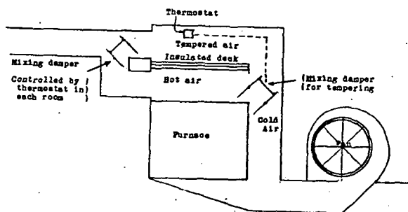
FIG. 64. AN ARRANGEMENT FOR TEMPERED AIR WITH WARM AIR FURNACES
