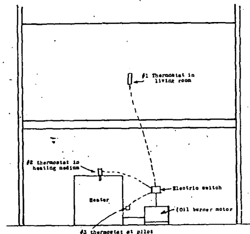
FIG. 66. TYPICAL ARRANGEMENT FOR OIL BURNER
