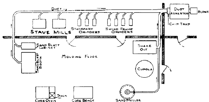
Fig. 4. Floor plan showing layout of equipment including stave mills.
