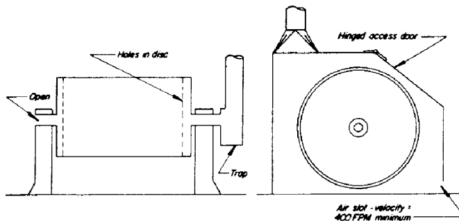
SECTION THRU HOLLOW TRUNNION TUMBLER
