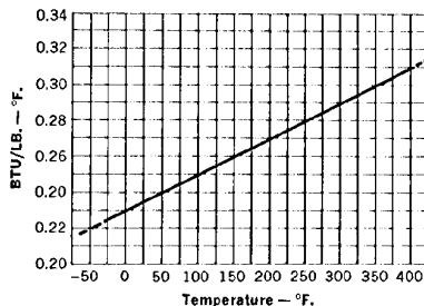
THERMINOL® FR Lo-Temp Specific Heat
