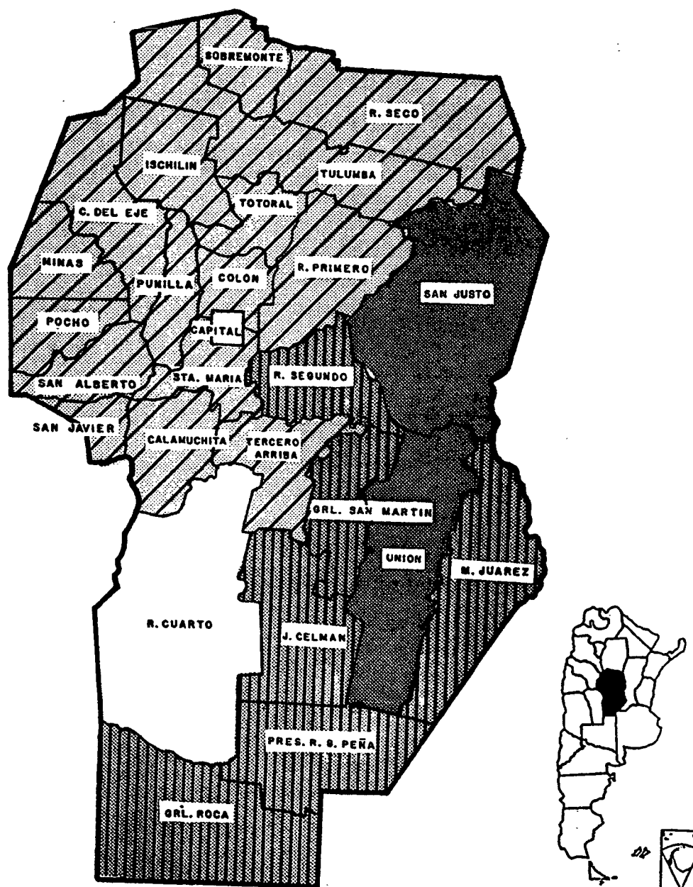
Figure 1 Map of Córdoba, Argentina, subdivided into counties and exposure categories; low-exposure group = diagonal lines; medium-exposure group = vertical lines; high-exposure group = gray; excluded from exposure classification = white
