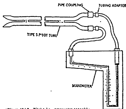
Figure 104-2. Pilot tube - manometer assembly.
