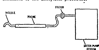
Figure 103-1. Beryllium screening method: sample train schematic.
