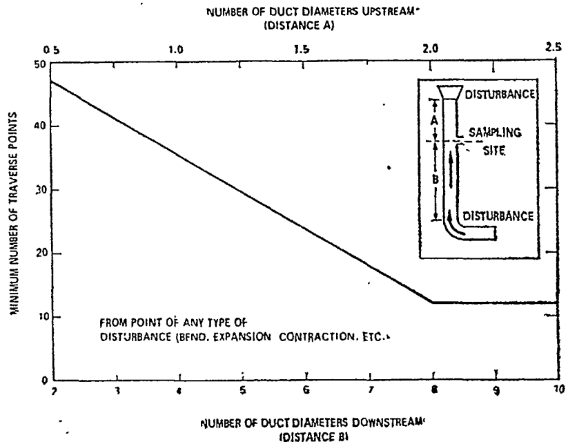
Figure 101-3. Minimum number of traverse points.
