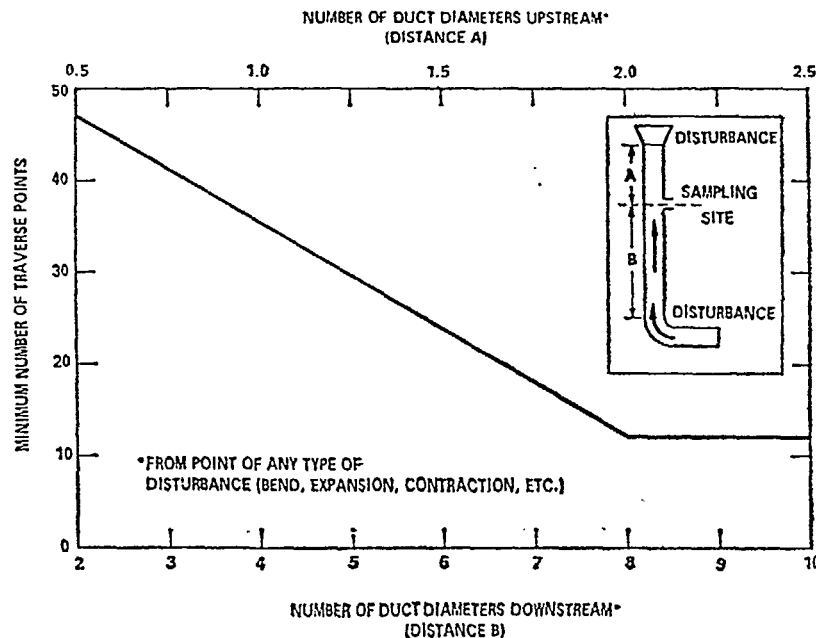
Figure 104-3. Minimum number of traverse points.
