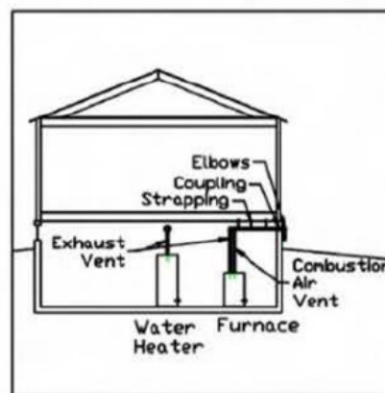
Figure 8D.3.3 Plastic PVC Installation (Condensing Example)
