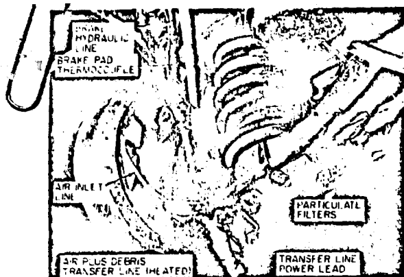
1. Disc brake emissions collector (left) from back, showing instrumentation; (right) showing thermal control aids.
