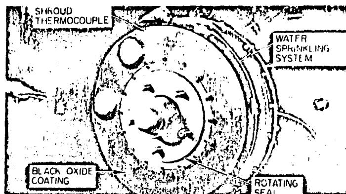
1. Disc brake emissions collector (left) from back, showing instrumentation; (right) showing thermal control aids.
