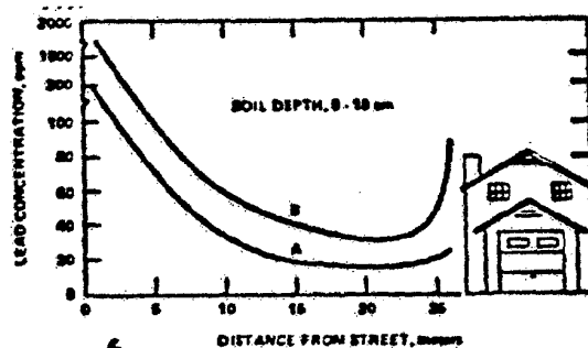
Figure C-6. Soil transacts by two streets: Curve A = low-traffic-volume (400 veh/day); Curve B = high-traffic-volume (14,000 veh/day). 20
