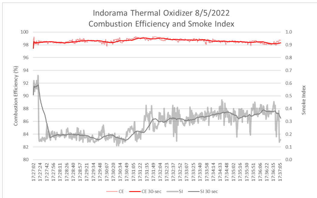
Figure 4: Combustion Efficiency and Smoke Index for the Thermal Oxidizer on 8/5/2022.
