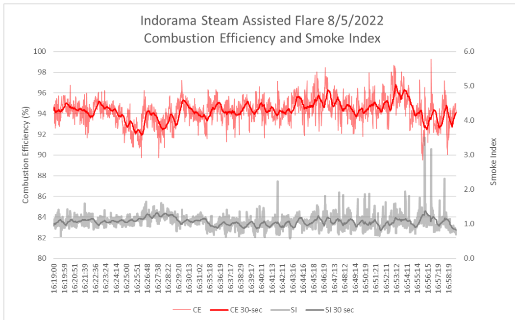
Figure 2: Combustion Efficiency and Smoke Index for the Steam Assisted flare on 8/5/2022.
