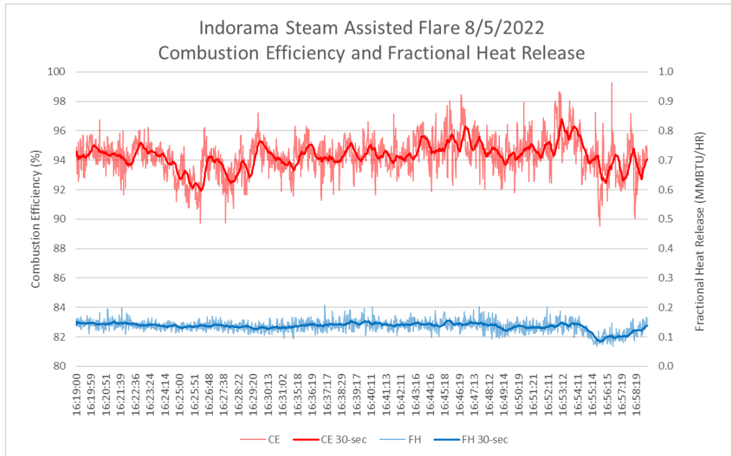
Figure 1: Combustion Efficiency and Fractional Heat Release for the Steam Assisted flare on 8/5/2022.
