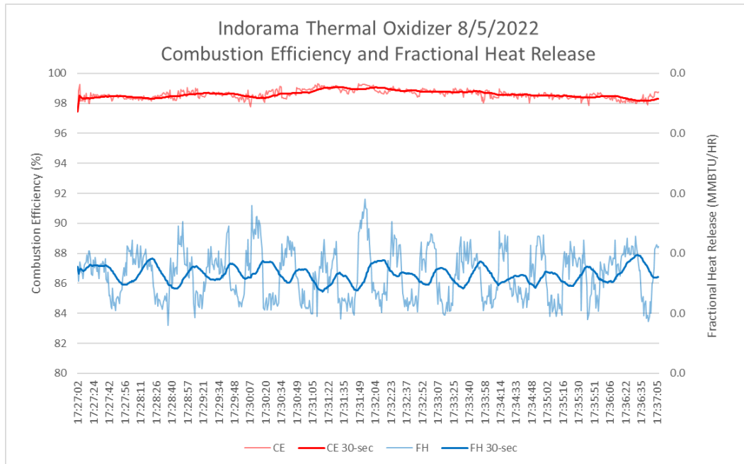
Figure 3: Combustion Efficiency and Fractional Heat Release for the Thermal Oxidizer on 8/5/2022.
