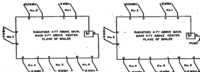
FIG. 10. ONE-PIPE GRAVITY CIRCULATION SYSTEM (EXAMPLE 3)
