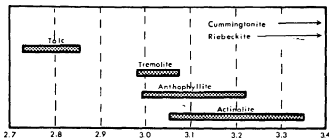
FIGURE 2. Specific gravities of talc and amphibole ( \rho ).
