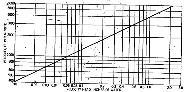
FIG. 4. RELATION BETWEEN VELOCITY AND VELOCITY HEAD FOR STANDARD AIR
