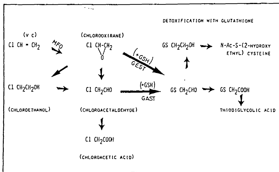
FIG. 1. The proposed metabolic fate of vinyl chloride. (GSH, glutathione; MFO, mixed-function oxidase; VC, vinyl chloride; GST, glutathione S-epoxide transferase; and GAST, glutathione S-aldhyde transferase).
