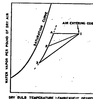
FIG. 12. PERFORMANCE OF DEHUMIDIFYING COIL
