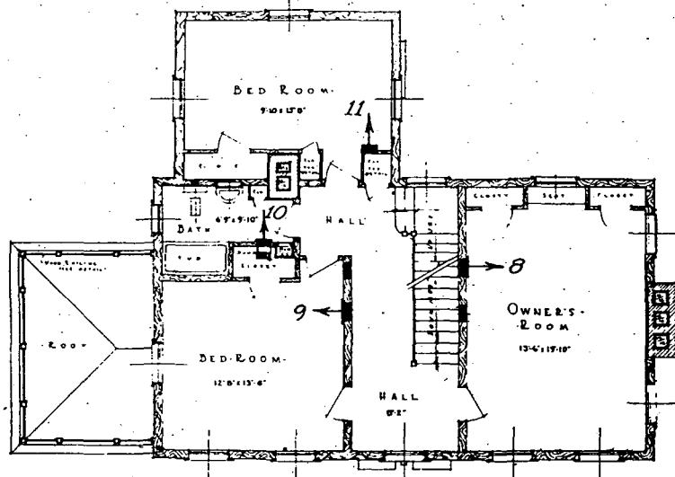
FIG. 58. SECOND FLOOR PLAN
