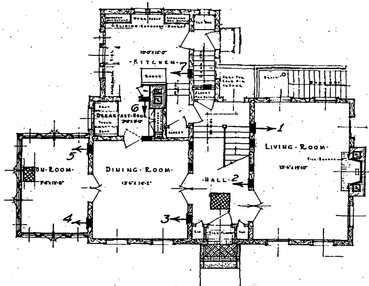
FIG. 57. FIRST FLOOR PLAN
