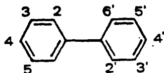
BIPHENYL MOLECULE AND RING NUMBERING SYSTEM
