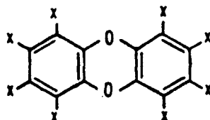
Chlorinated Dibenzodioxin
