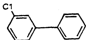
3-chlorobiphenyl
