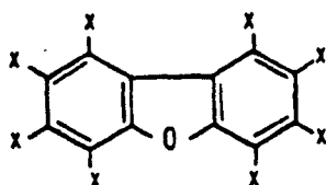
Chlorinated Dibenzofurans
