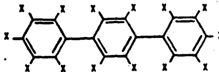
Polychlorinated Terphenyls
