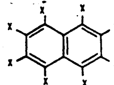
Polychlorinated Naphthalenes
