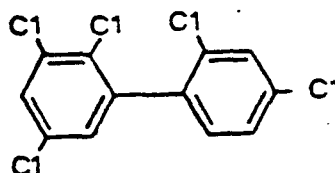
2,2',3,4',5-pentachlorobiphenyl
