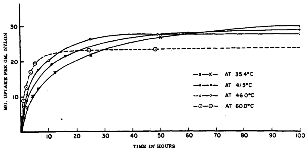
Fig. 17.—Effect of temperature on the sorption of salicylic acid by nylon. [From Kapadia, A. J., Guess, W. L., and Autian, J., "Sorption and Diffusion Studies of Salicylic Acid in a Nylon Sheet," to be published.]
