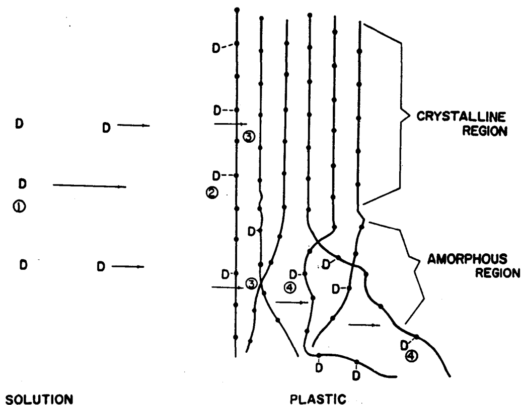
Fig. 10.—A schematic model showing sorption of a drug by nylon. D = drug molecule; -- = polymer chain; and • = binding sites in polymer.
