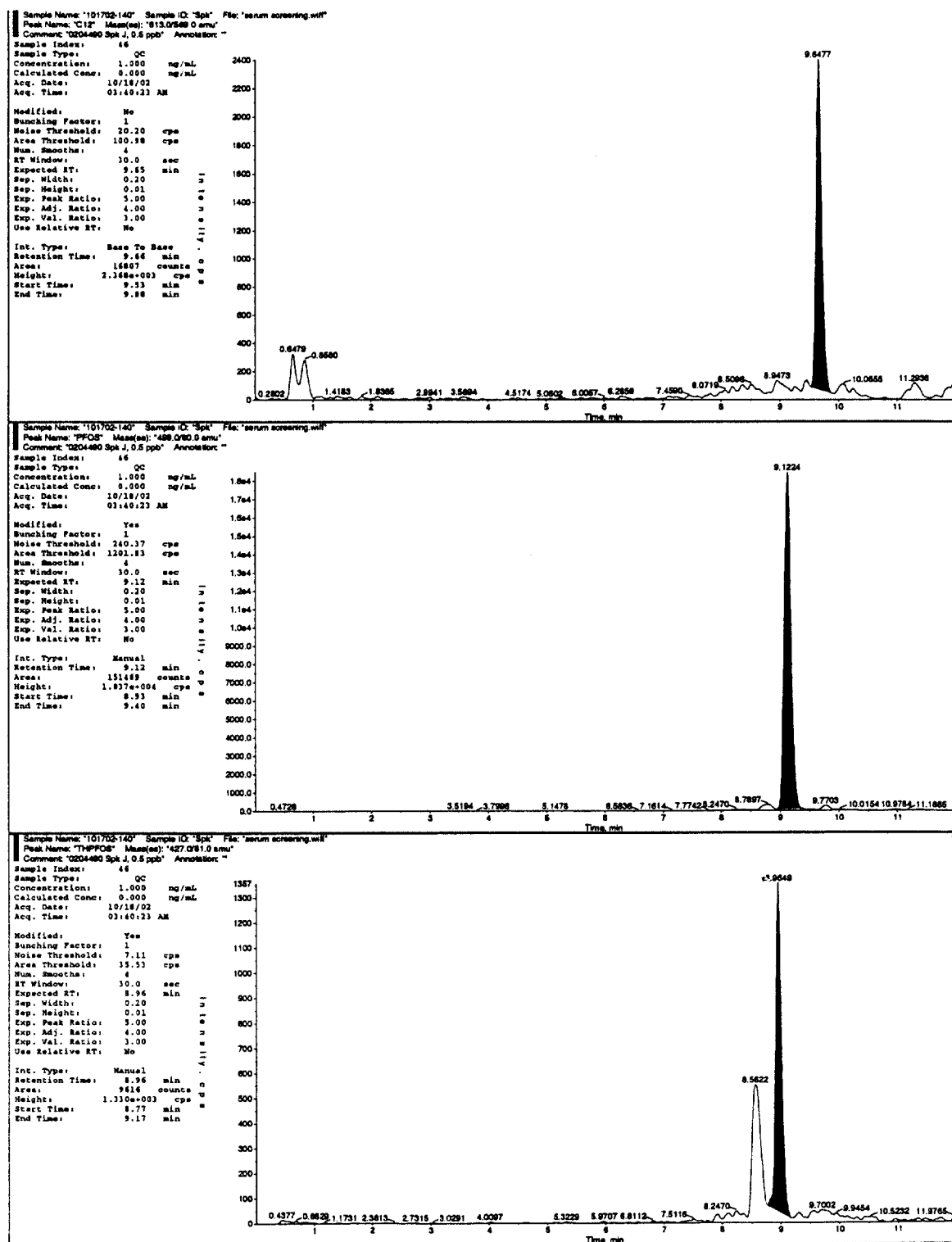
Figure 2 (cont') Chromatogram Representing a Fortified Human Plasma Sample at 0.5 ppb (Exygen ID: 0204490 Spk J, Sponsor ID: TCR-674)
