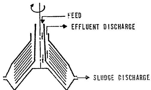
DISC TYPE CENTRIFUGE
