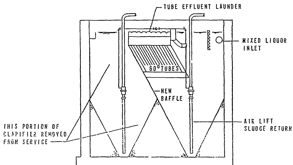
FIGURE 6-3 INSTALLATION OF TUBE SETTLERS AT THE WICKAM, PENNSYLVANIA SEWAGE TREATMENT PLANT (20)
