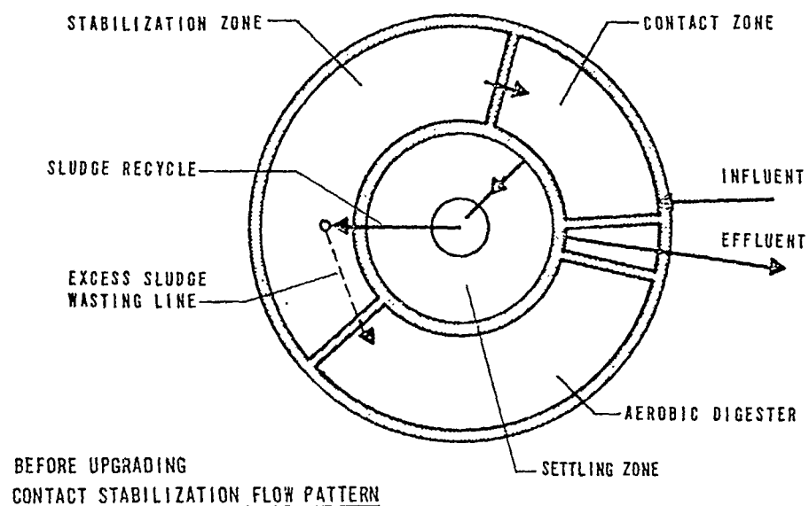
FIGURE 13-6 CASE HISTORY NO. 5 UPGRADING A CONTACT STABILIZATION PACKAGE PLANT TO A COMPLETELY-MIXED FLOW PATTERN (5)
