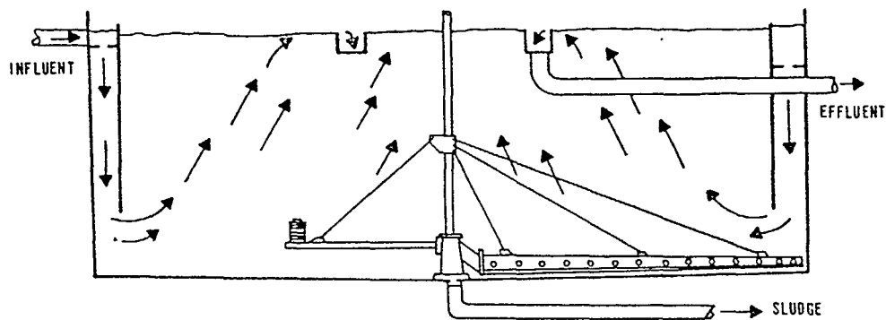
CIRCULAR PERIPHERAL FEED CLARIFIER WITH A HYDRAULIC SUCTION SLUDGE REMOVAL SYSTEM
