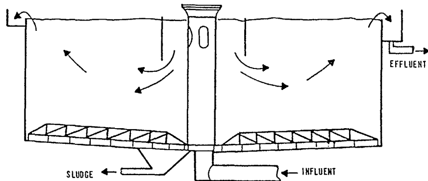
CIRCULAR CENTER FEED CLARIFIER WITH A SCRAPER SLUDGE REMOVAL SYSTEM
