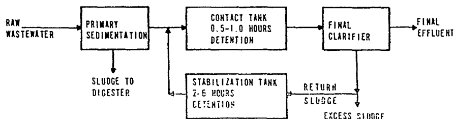
FIGURE 5-4 CONTACT STABILIZATION FLOW DIAGRAM
