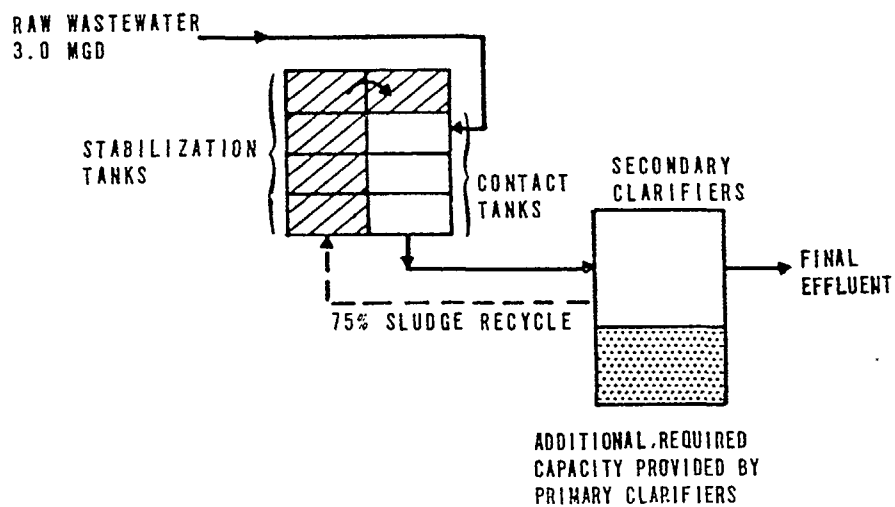
TREATMENT SYSTEM AFTER UPGRADING CONTACT STABILIZATION PROCESS
