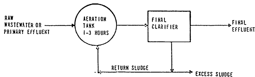
FIGURE 5-5 COMPLETELY-MIXED FLOW DIAGRAM
