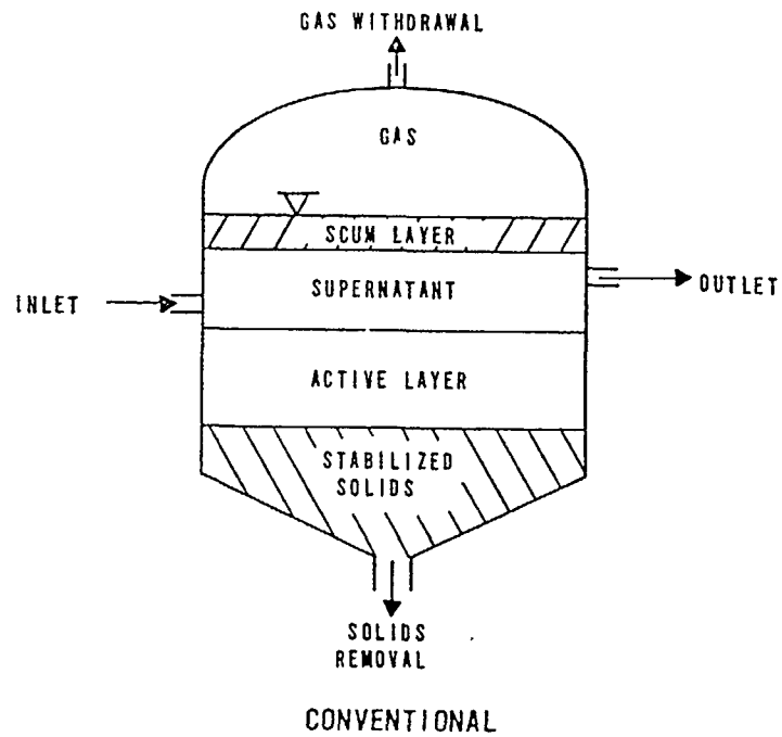
FIGURE 11-2 DIGESTION SYSTEMS
