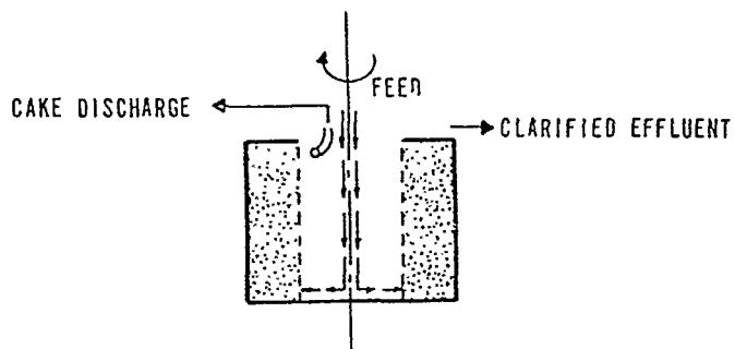
SOLID BOWL BASKET CENTRIFUGE
