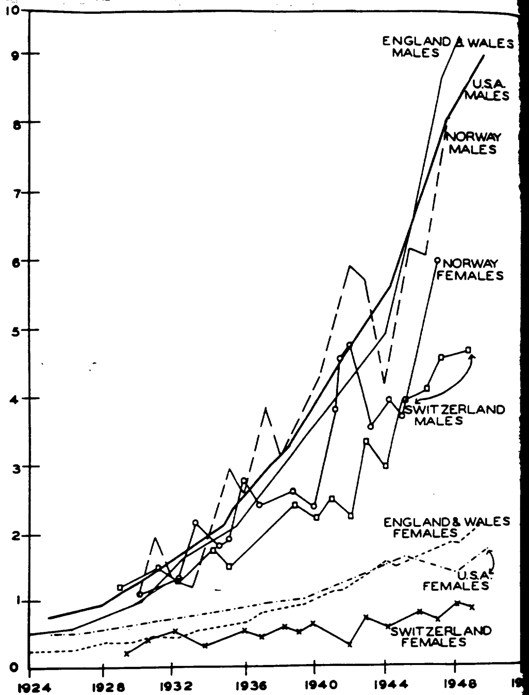
Figure 1. Comparative trends in respiratory cancer mortality, 1924-50.
