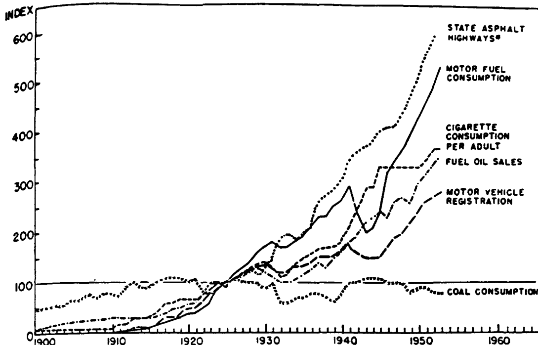
Figure 2. Trends in selected environmental factors, United States, 1900-53 (Hammond).
