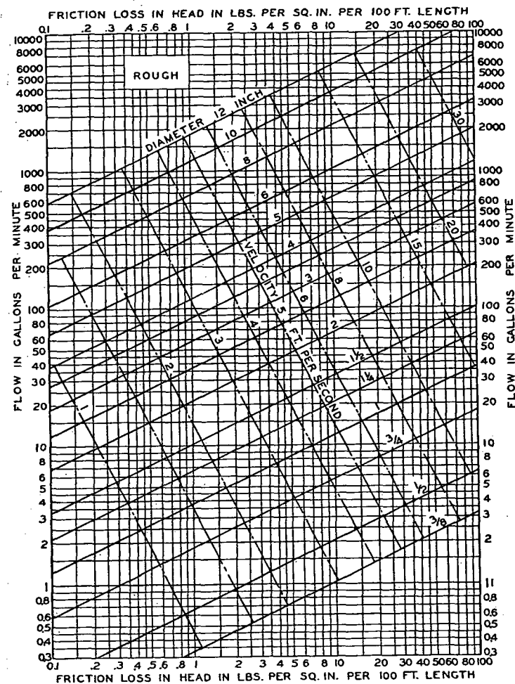
Fig. 5....Flow Chart for Rough Pipe 1
