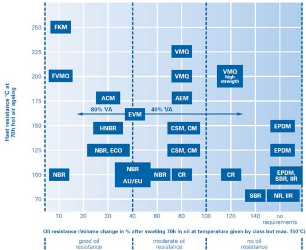
Classification of elastomers according its heat and oil resistance following ASTM D 2000 (issue 2006)
