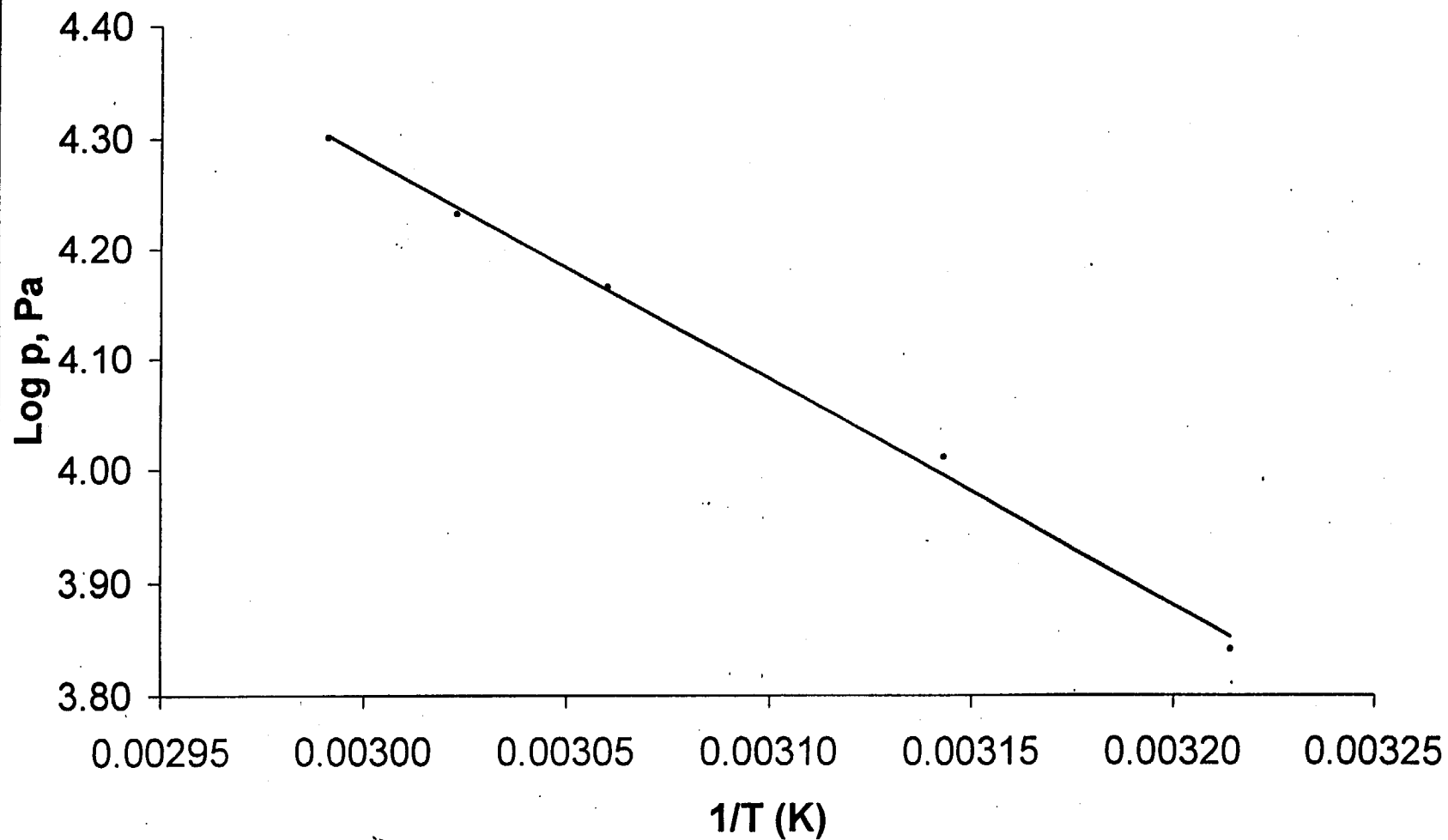
Figure 2. A Representative Plot of Log p (Pa) and 1/T (K) for Toluene at Decreasing Pressure
