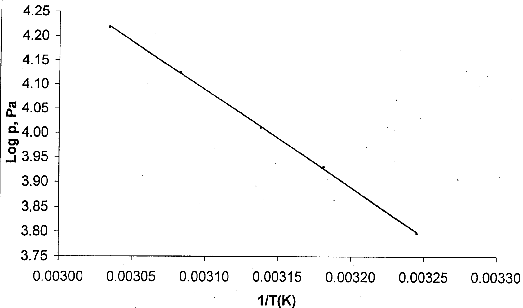
Figure 1. A Representative Plot of Log p (Pa) and 1/T (K) for Toluene at Increasing Pressure
