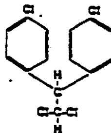
DDD
