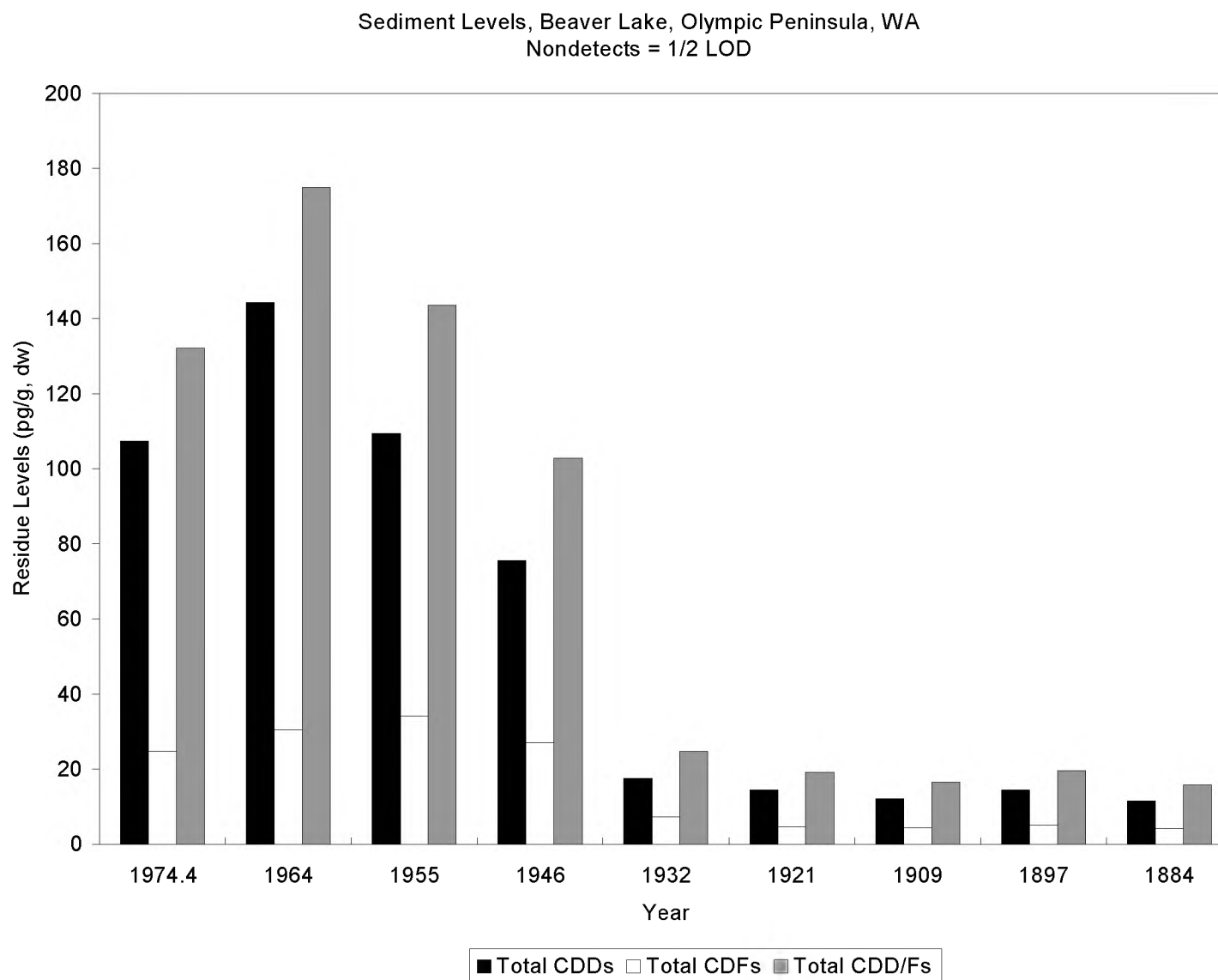
Figure 6-1. CDD/CDF Levels in Sediment, Beaver Lake, Washington
