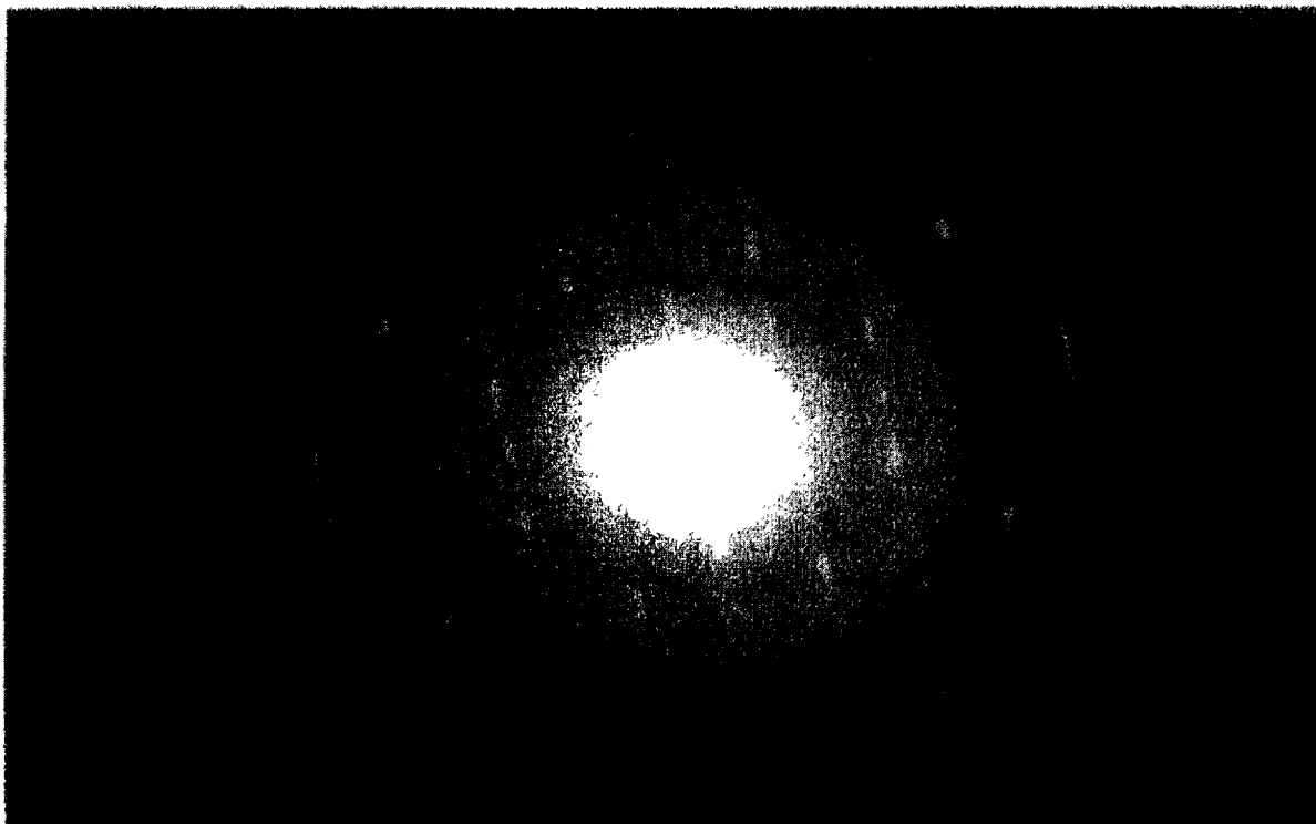
FIG. I. Electron diffraction pattern of a chrysotile fiber.
