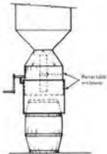
Dust Enclosure for Drum-Filling Operation
