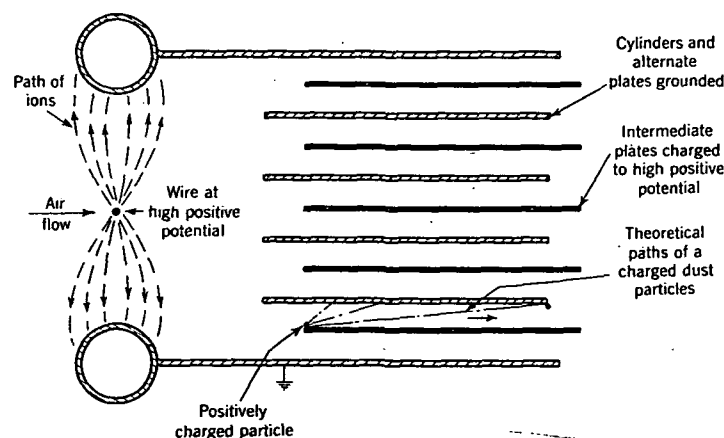
FIG. 4. DIAGRAMMATIC CROSS-SECTION OF ELECTROSTATIC PRECIPITATOR
