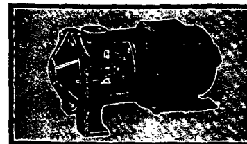
Fig. 2130—Close-Coupled, side suction pump. Capacities range from 2 to 500 Gpm against heads up to 189 ft. Motors from 1/8 to 20 H.P. Discharge 1 to 3 in. Closed and open type impellers. Bulletin 108.
