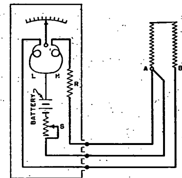
FIG. 2. TYPICAL RESISTANCE THERMOMETER CIRCUIT AND CONNECTIONS
