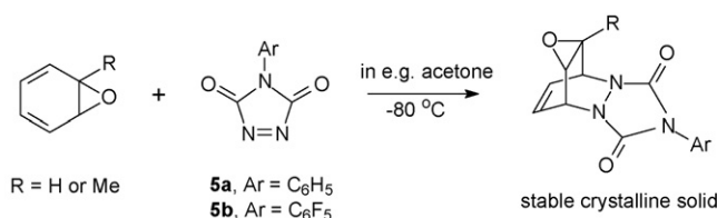
Scheme 5. Reaction of benzene oxide-oxepin and toluene oxide-2-methyloxepin with 4-phenyl-1,2,4-triazoline-3,5-dione (Cookson's dienophile, 5a ) and its pentafluoro analogue 5b .
