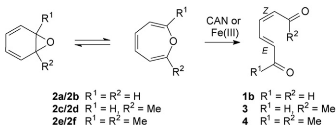
Scheme 1. Conversion of arene oxides-oxepins to ( E,Z )-muconaldehydes [CAN=cerium(IV) ammonium nitrate; Fe(III)=iron(III) tris (1,10-phenanthroline) hexafluorophosphate].
