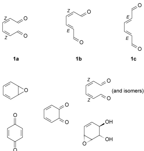
Fig. 1. Some reactive benzene metabolites.
