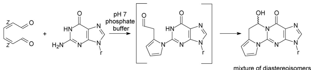
Scheme 4. Reaction of ( Z,Z )-muconaldehyde with guanosine derivatives leading to pyrrole adducts ( r = \text{ribose or deoxyribose} ).
