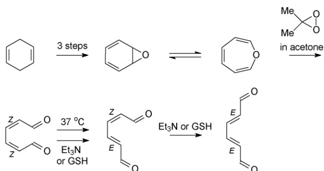
Scheme 2. Synthetic routes to isomeric muconaldehydes.
