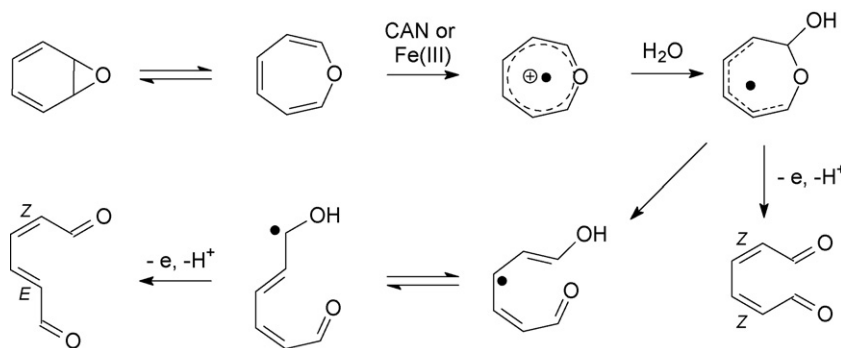
Scheme 3. Putative mechanism of oxidation of 2a/2b by CAN or Fe(III) to 1b .
