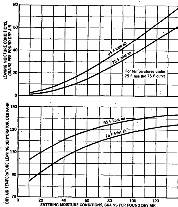
FIG. 7. SILICA GEL DEHYDRATOR PERFORMANCE DATA
