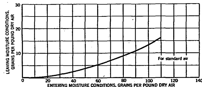
FIG. 8. ACTIVATED ALUMINA DEHYDRATOR PERFORMANCE DATA
